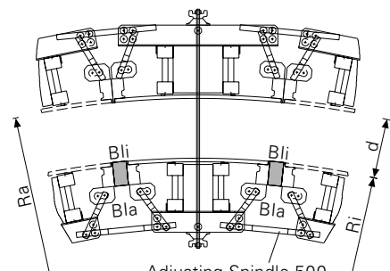
Adjusting Spindle 500
